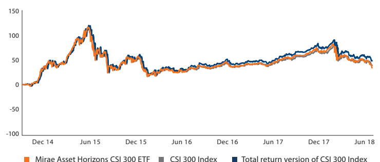
Cumulative performance (%)
